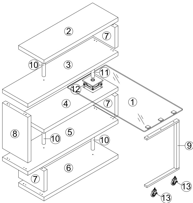
Exploded View
