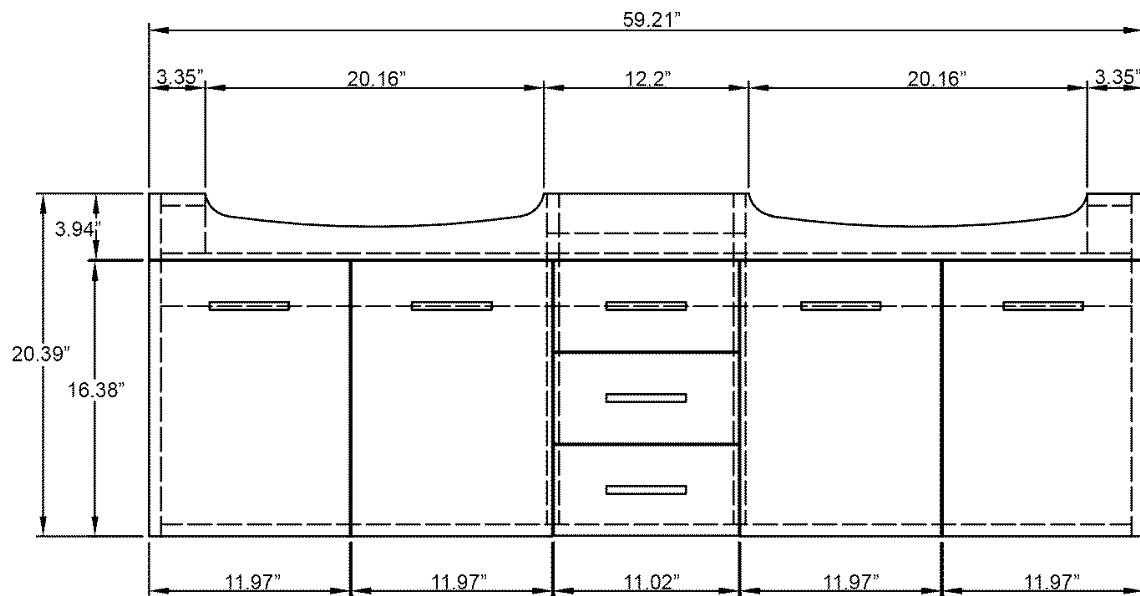
Front View
