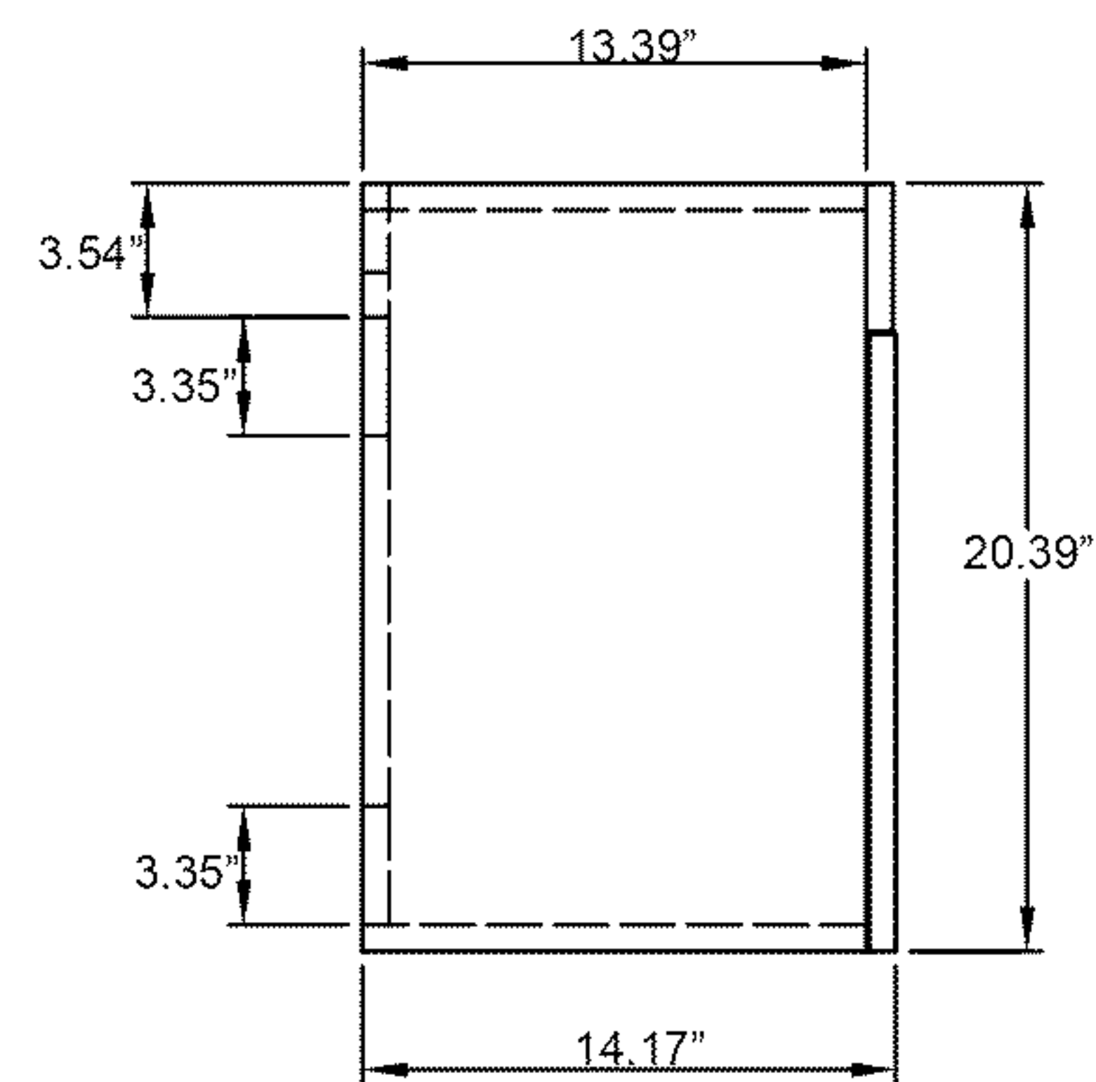
Side View
