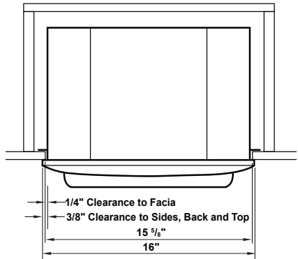
Figure 6 - Clearance to Combustibles
