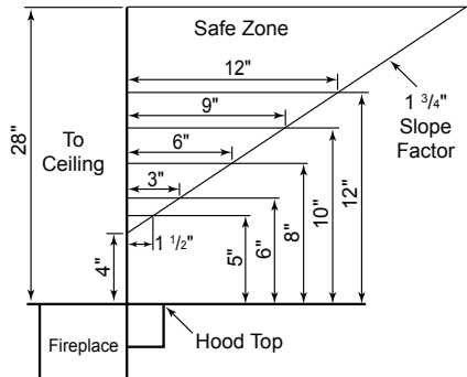
Figure 7 - Fireplace Clearances
