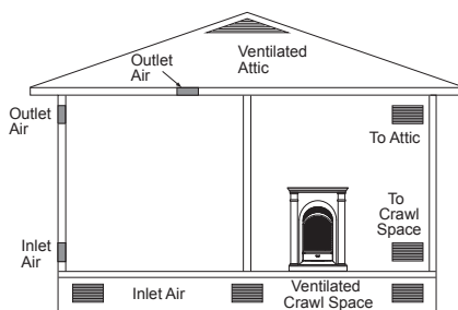
Figure 3 - Ventilation Air from Outdoors (Mantel installation shown)
