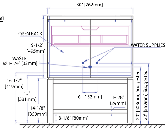
30" VANITY BACK VIEW (V8000 30)
