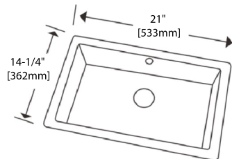
BASIN TOP VIEW (C09 2114)
