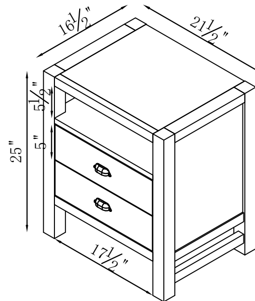
ANWI01 2 Drawer Bedside Nightstand
