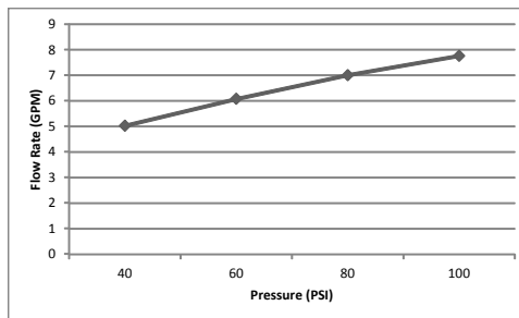
4021B Flow Rate (GPM) Vs Pressure (PSI)*
