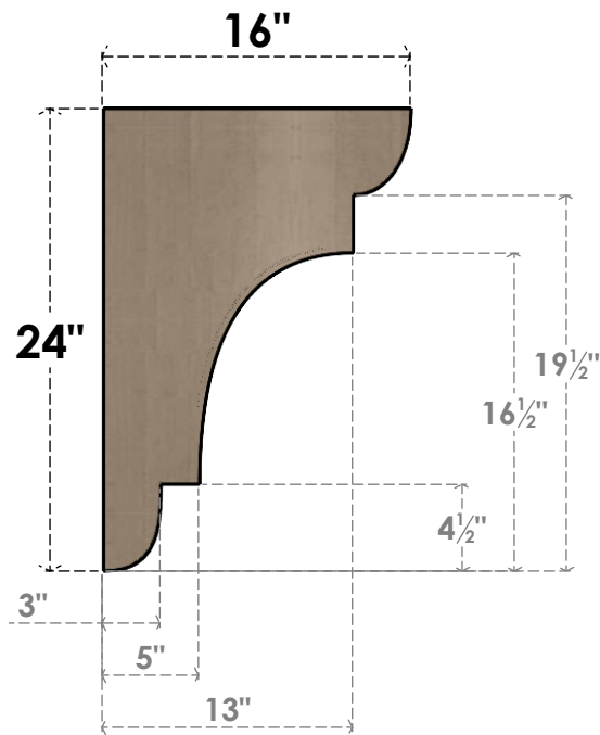
SIDE PROFILE
