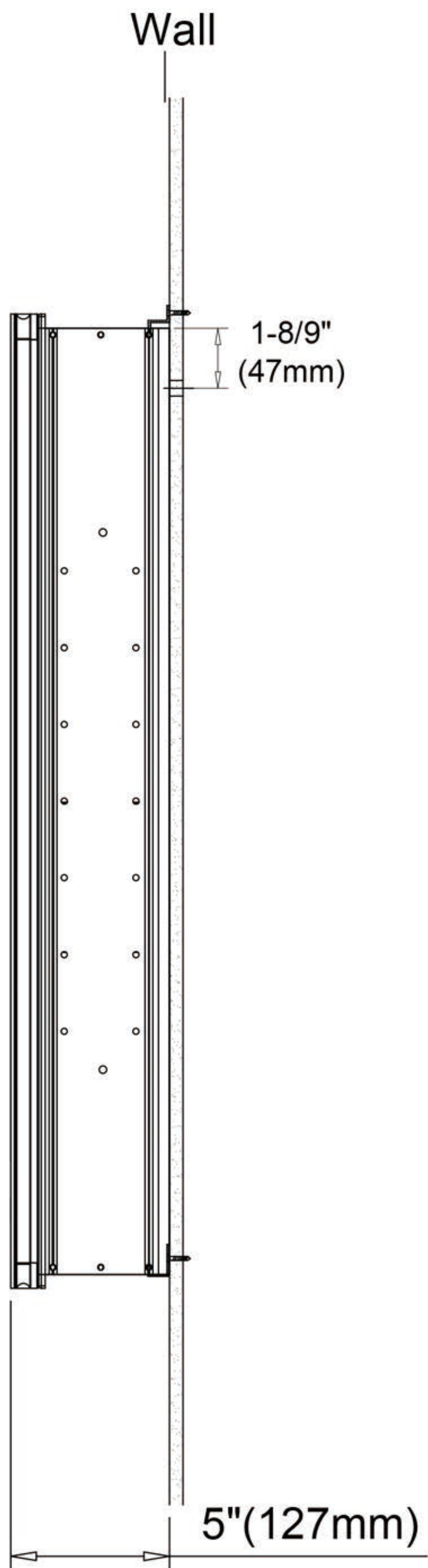
Surface Mount
