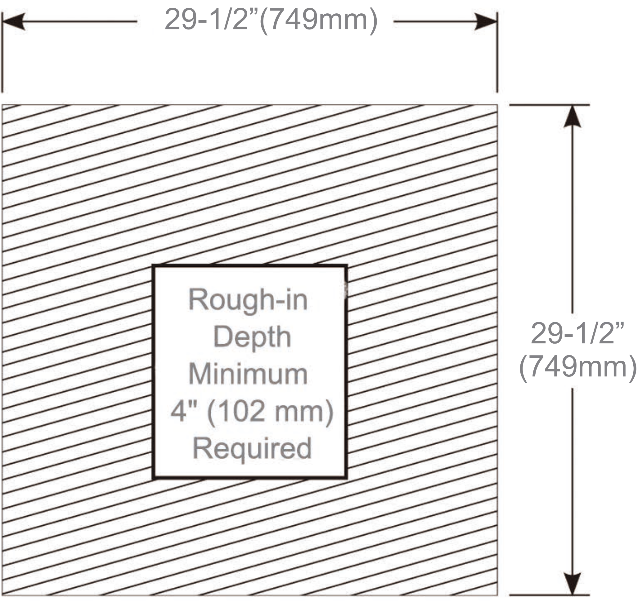
Rough-in Dimensions
