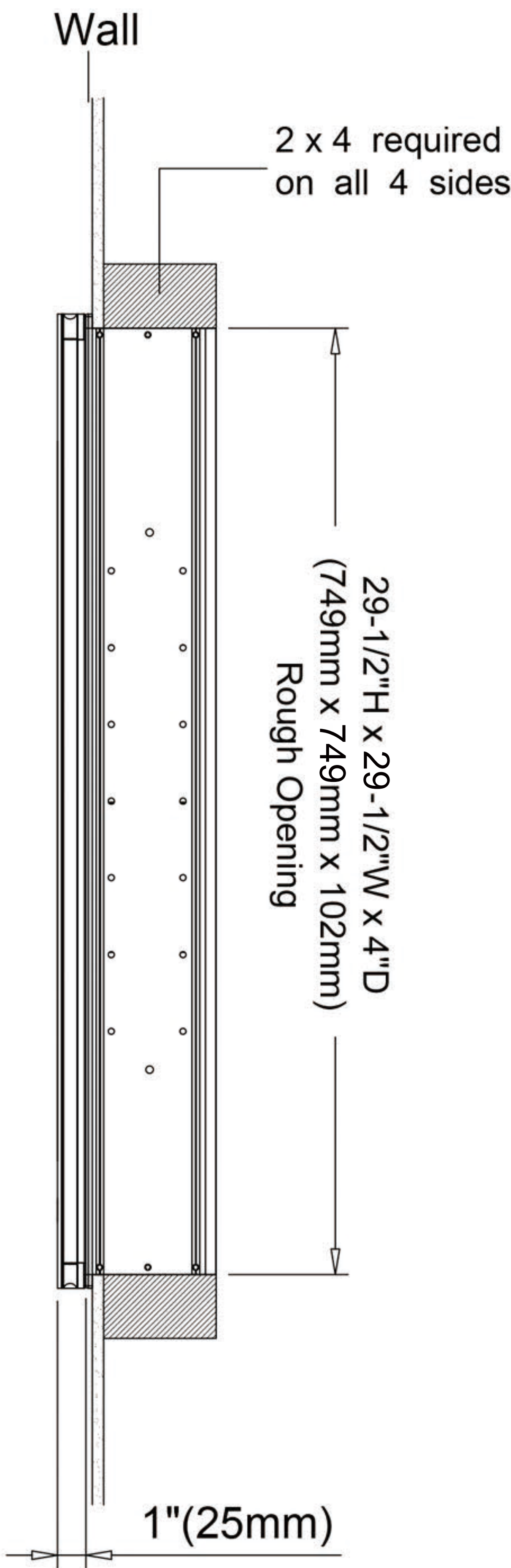
Recessed Mount
