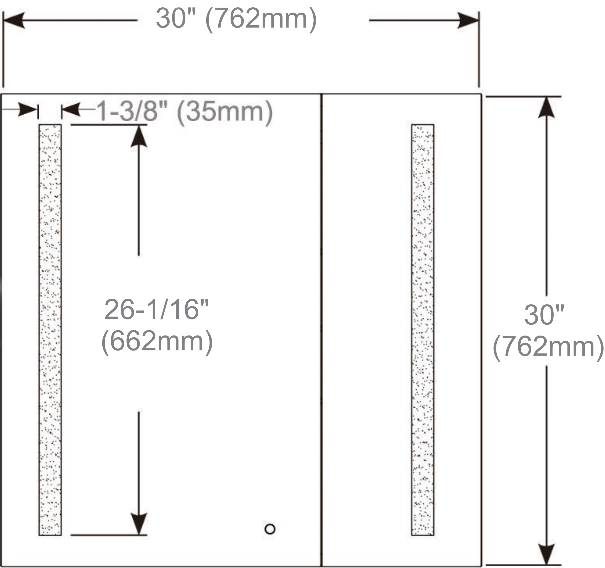
Cabinet Dimensions
