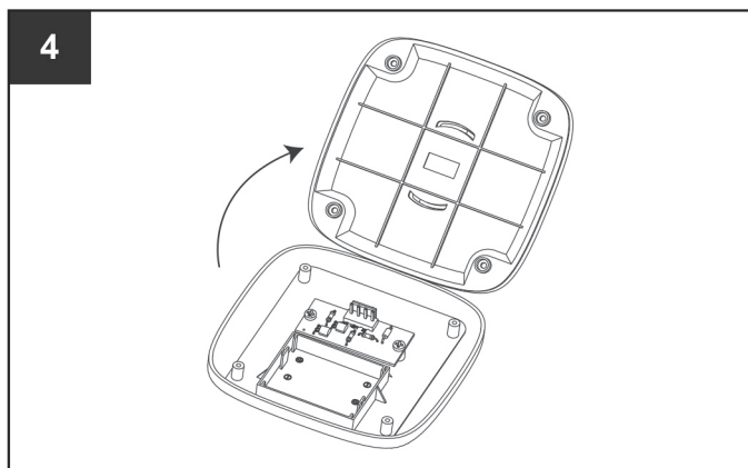
Step 4: Carefully open the bottom case and set aside. Replace the battery, matching the +/- on the battery with the +/- on the battery case.
