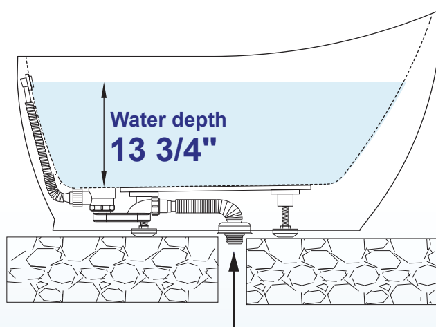
Anti-leak drain and pipe
