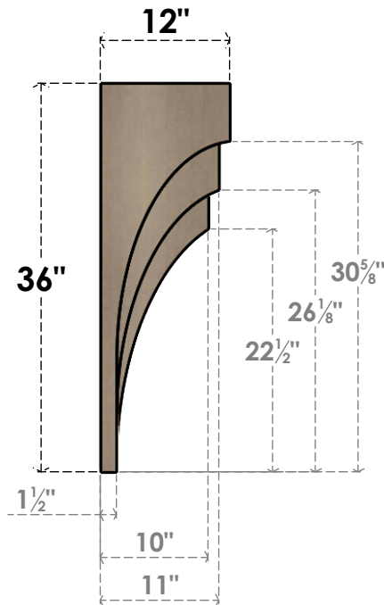
SIDE PROFILE
