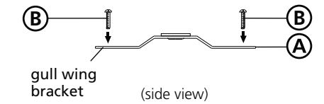
DRAWING 2 - MOUNTING
