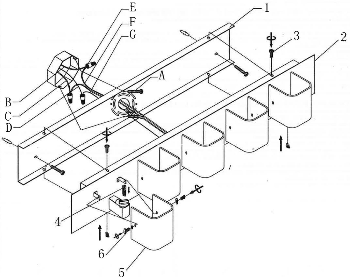
Wire connection
