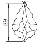
CC (double sided) 89mm Part: PT-CRYSTAL-1323-CC
