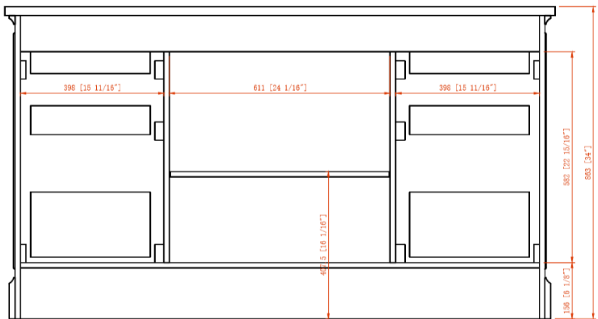
BACK VIEW
