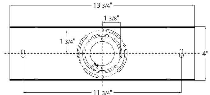
Back Plate Dimensions
