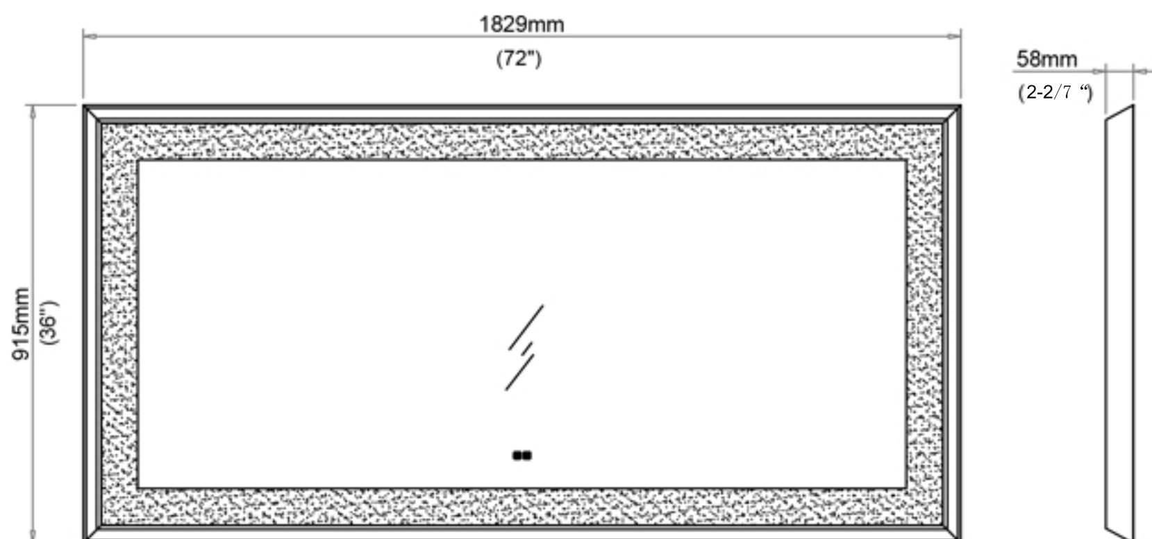
Front view
