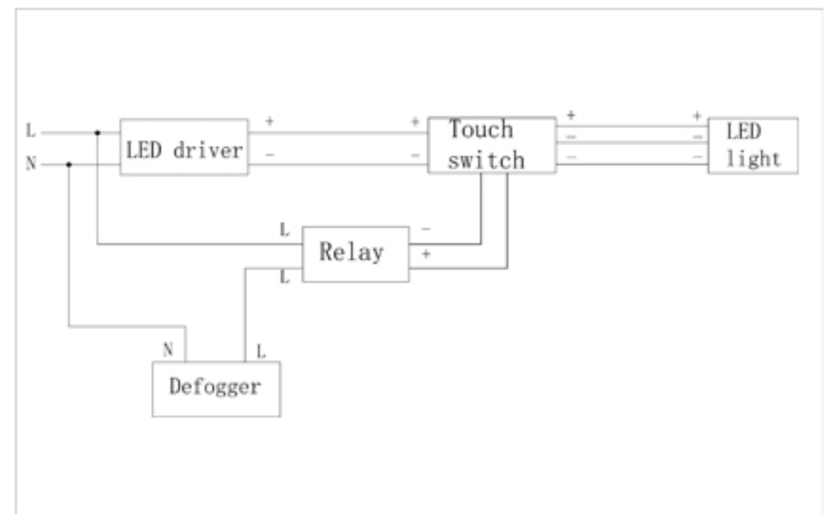
Circuit diagram
