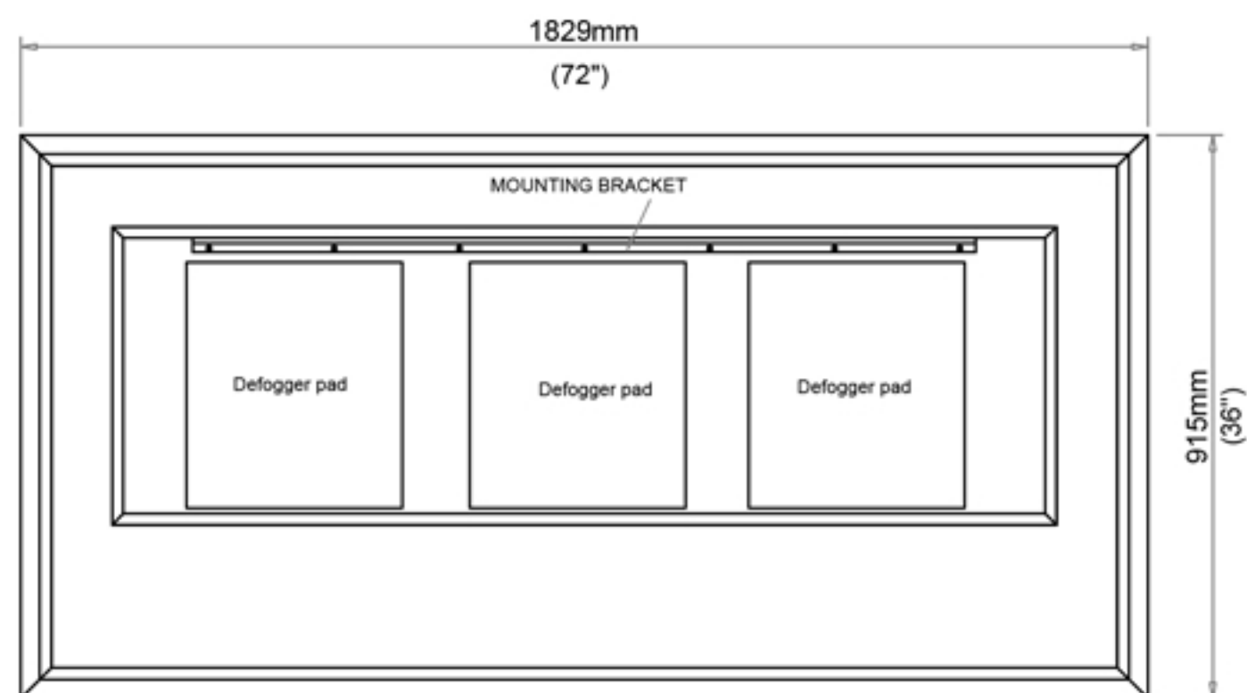
Back view for electrical knockout location
