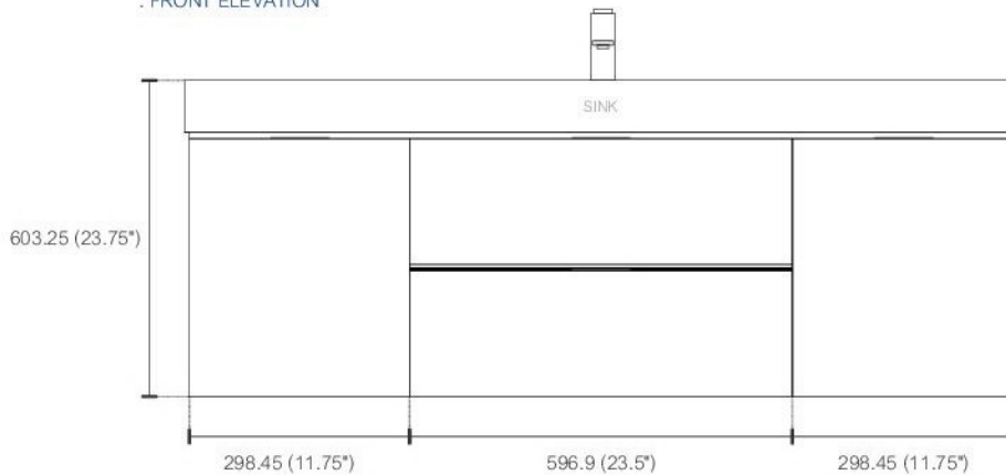
. FRONT ELEVATION
