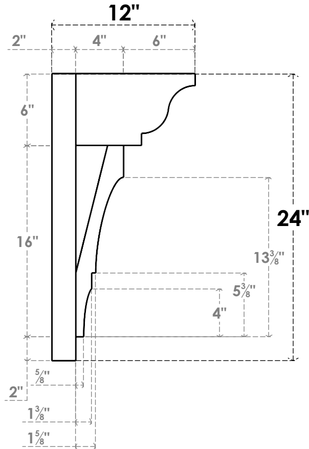
SIDE PROFILE
