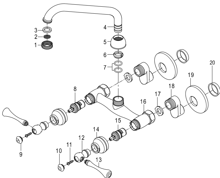
Cold Cartridge: KC1000C
