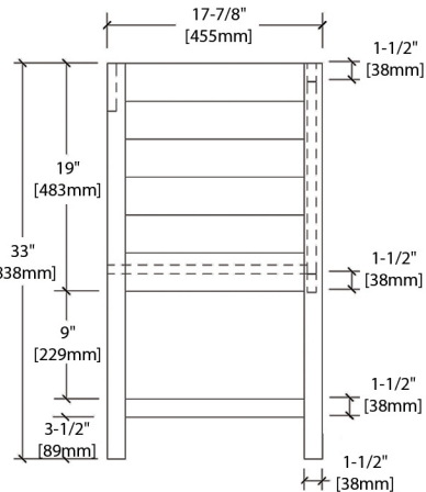
VANITY SIDE VIEW (V8017 30)
