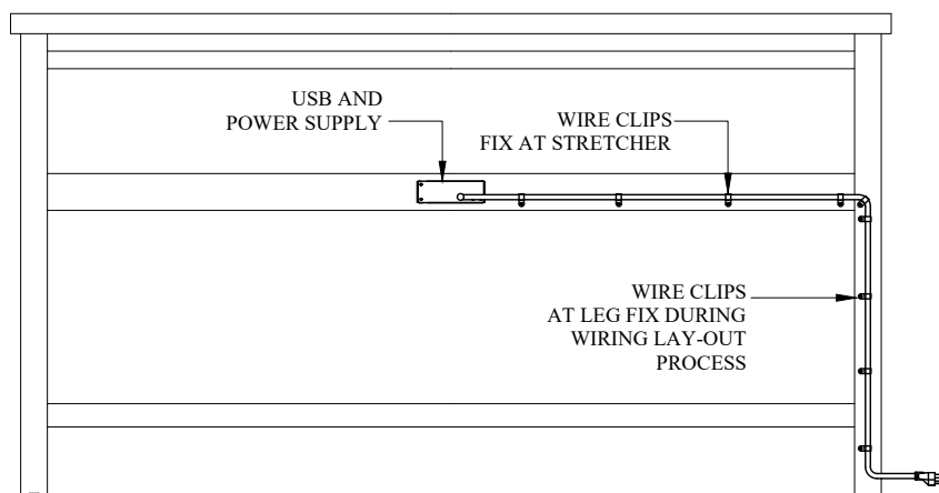
BACK VIEW SHOWING WIRING LAY-OUT OPTIONS
