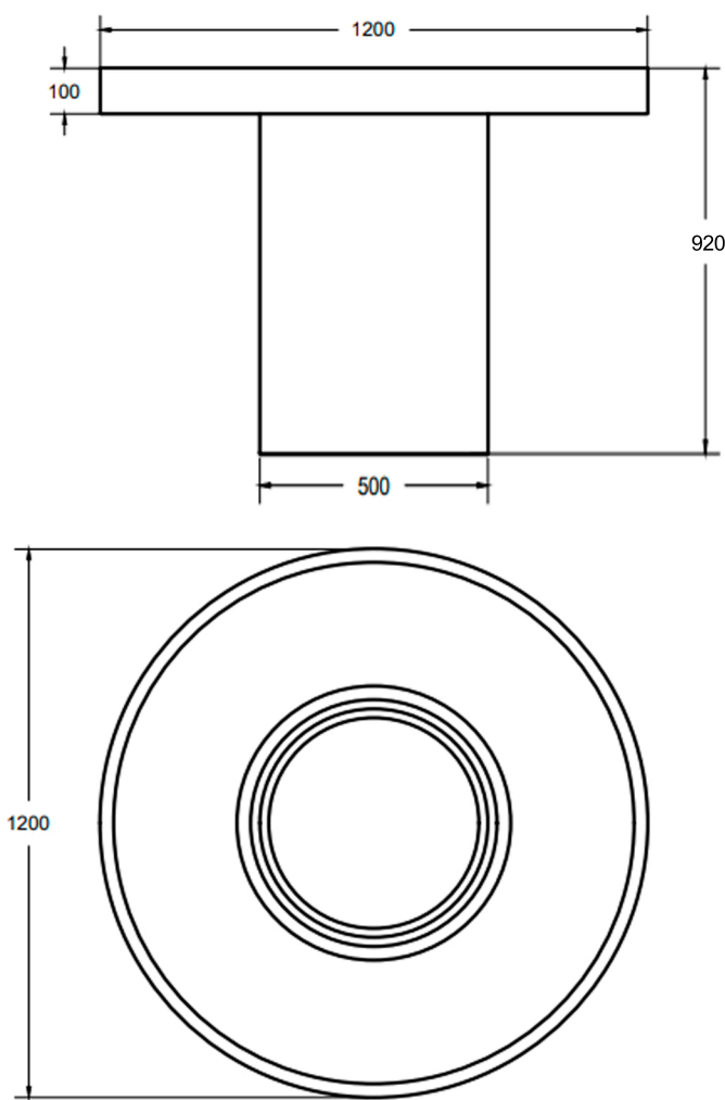
CIRCA TABLE - COUNTER HEIGHT VGS-CIRCA-DT-4-CNTR
