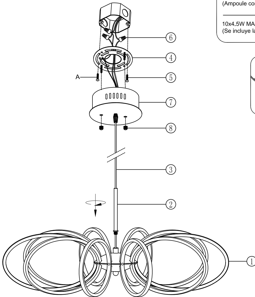
Wire connection
