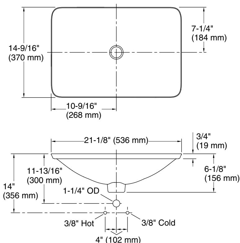
Standard Installation
