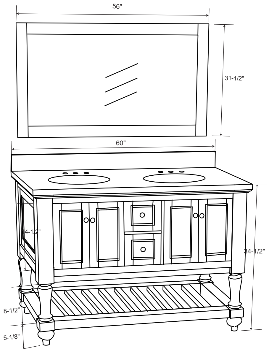
60" Front View
