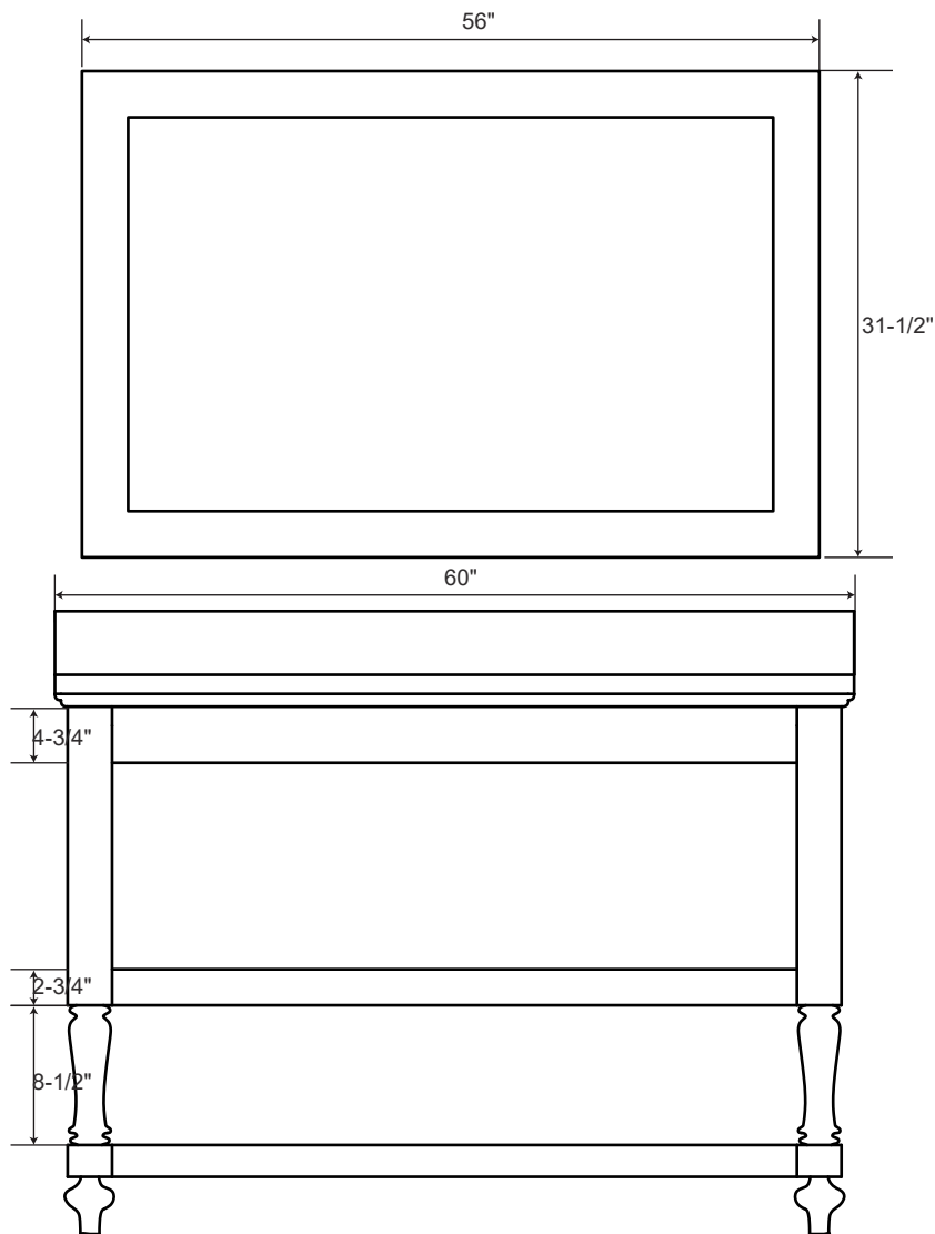
60" Back View
