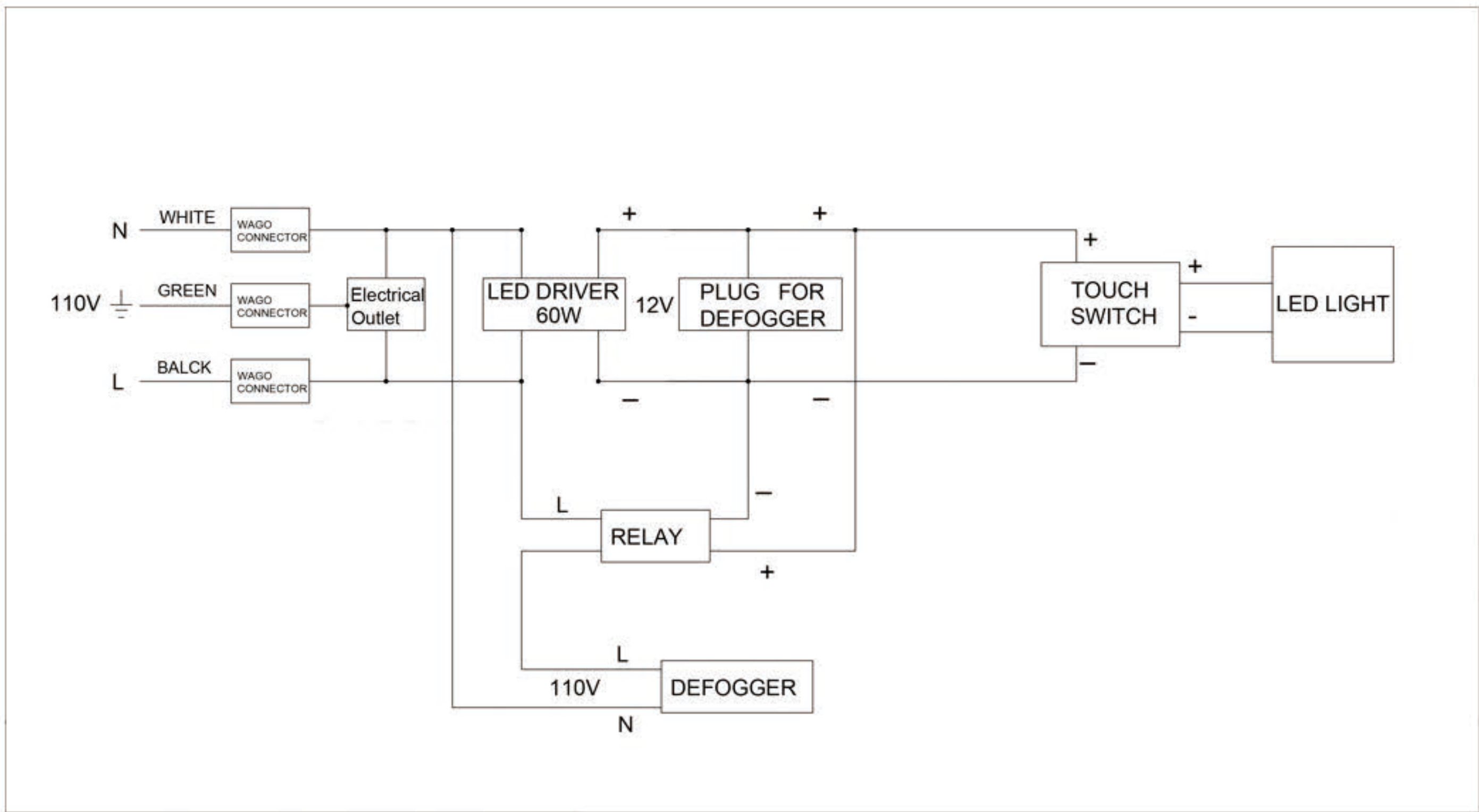
Circuit Diagram
