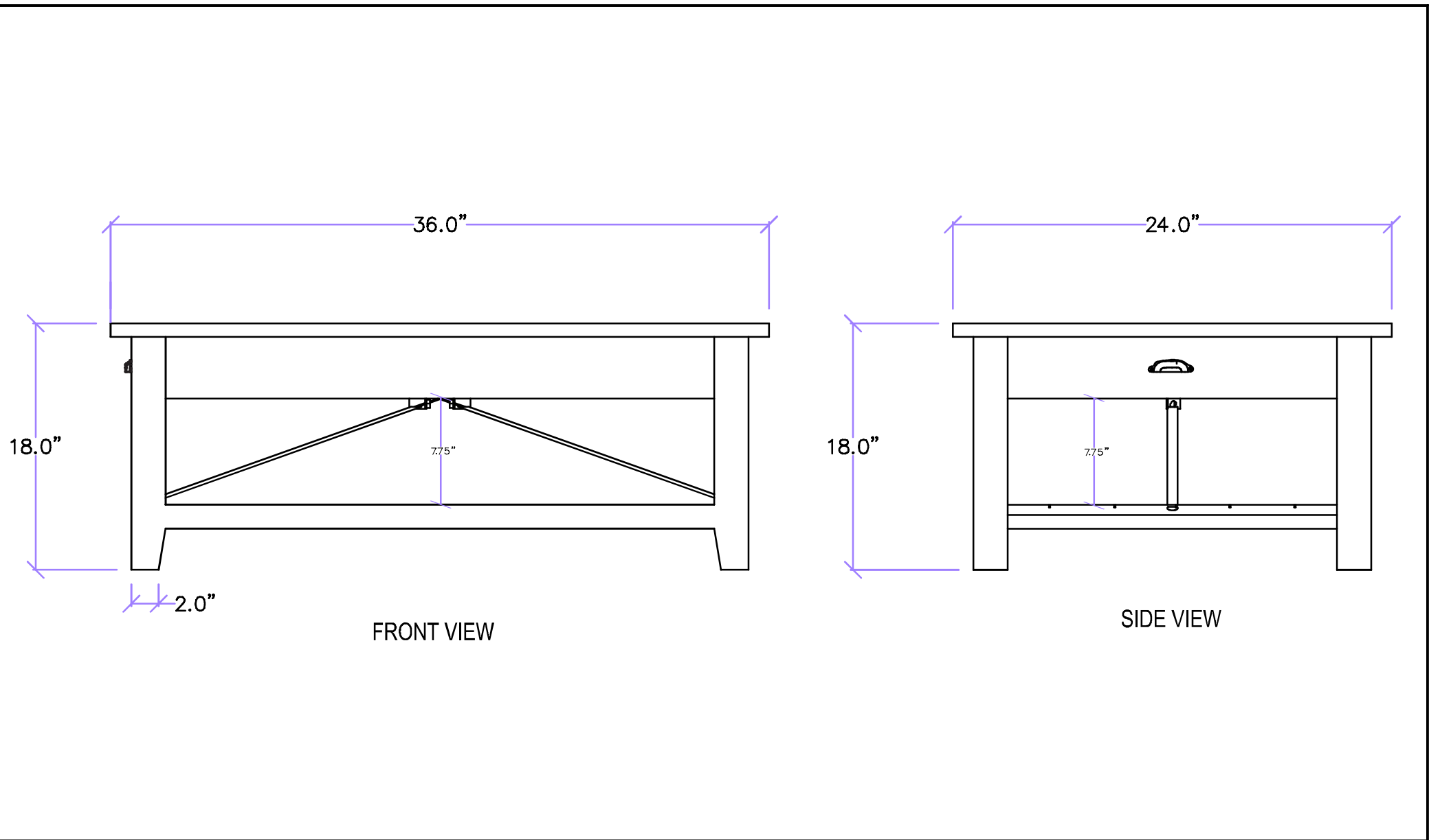
AWMW1371Z / MILLWORKS / ZINC TOP COFFEE TABLE 24" X 36" WITH DRAWER
