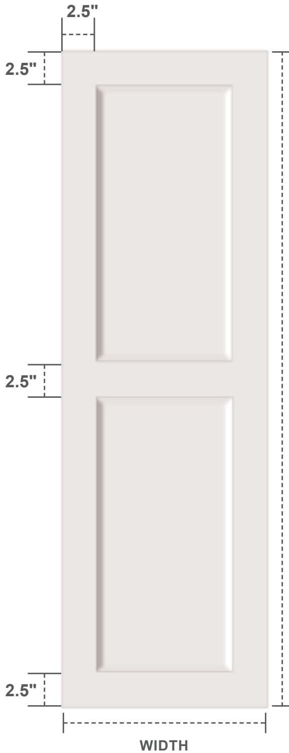
FRONT VIEW
