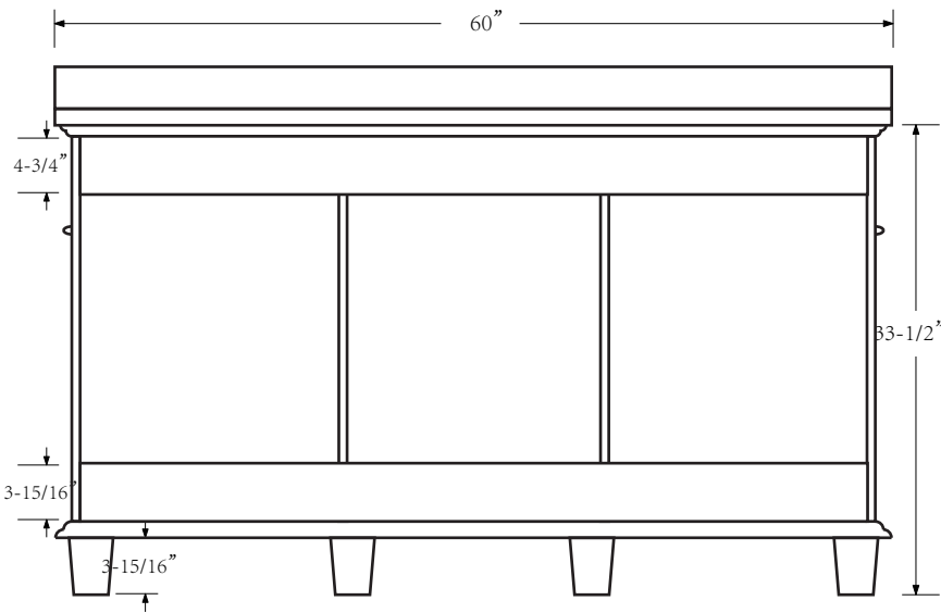
BACK VIEW
