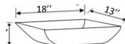
UNDERMOUNT SINK
