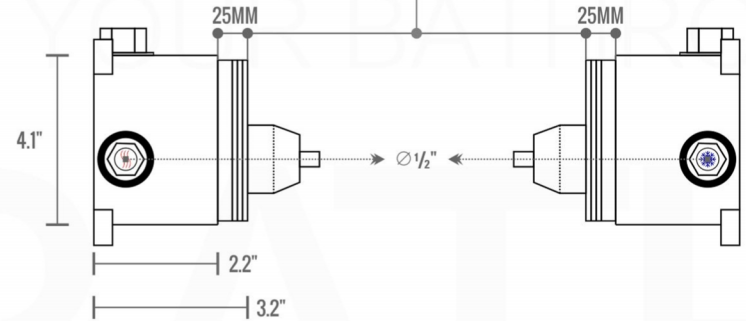
LEFT VIEW
