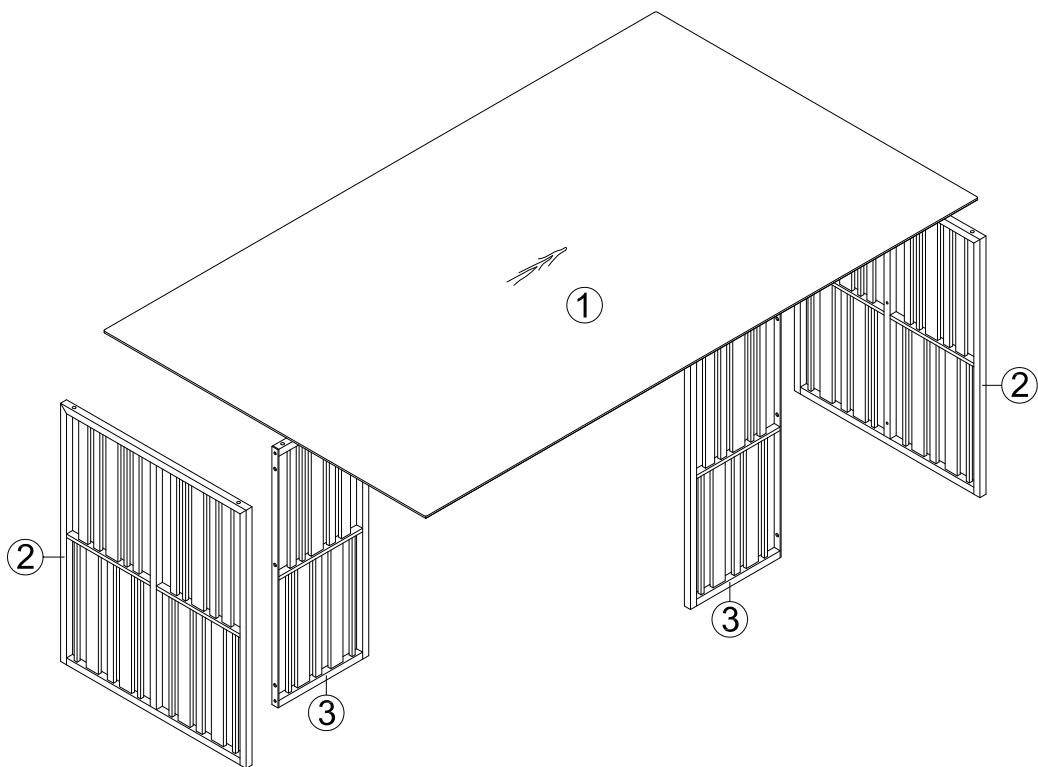
Exploded View
