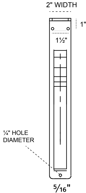
FRONT PROFILE
