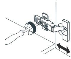
adjust depth
