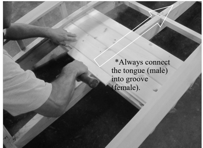
14. Continue to slide in more floor boards.
