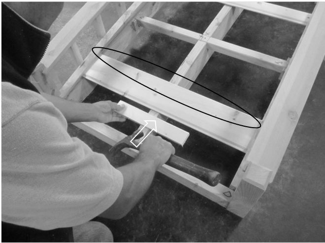
13. Check the tongue and groove of the end floor board on the other end and slide in floor boards one at a time. The tongue of the floor boards should go into the groove.
