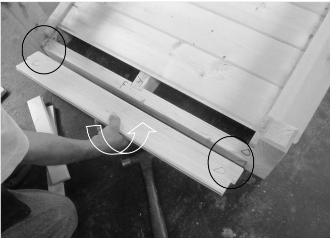
15. Put the end floor board. Match the number.
