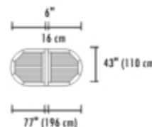
FULLY CLOSED
