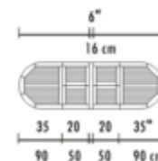
FULLY EXTENDED
