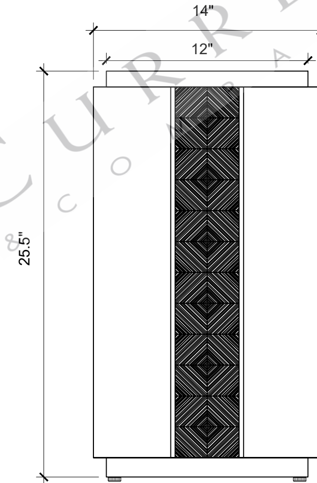
FRONT VIEW
