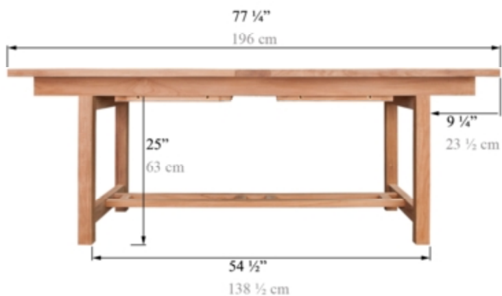
Front View FULLY CLOSED
