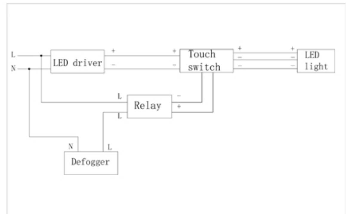
Circuit diagram
