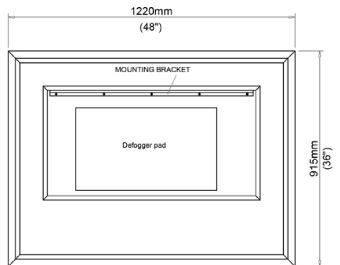
Back view for electrical knockout location
