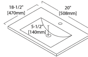
TOP-MOUNT BASIN (C04 2018)
