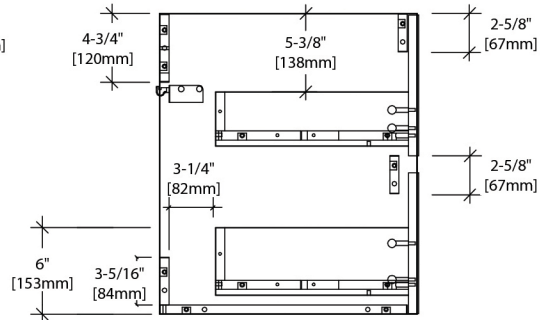
VANITY TOP VIEW (V8016 20)
