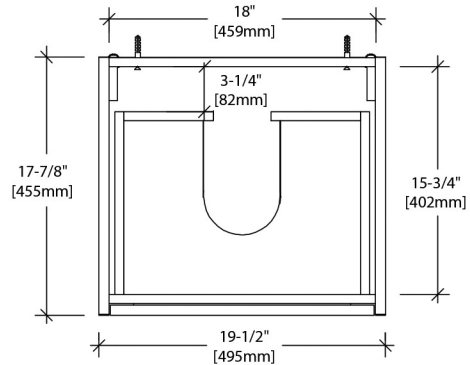
VANITY TOP VIEW (V8016 20)
