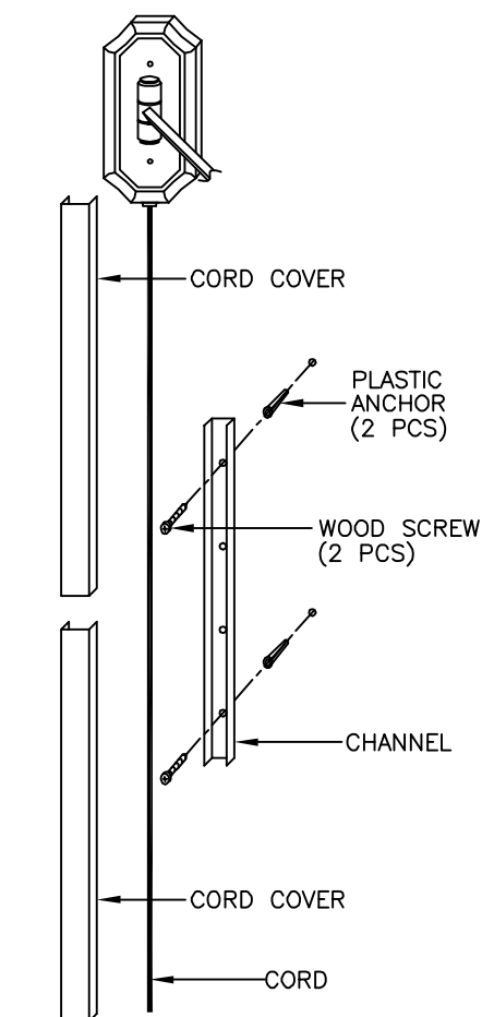
CORD COVER ASSEMBLY
