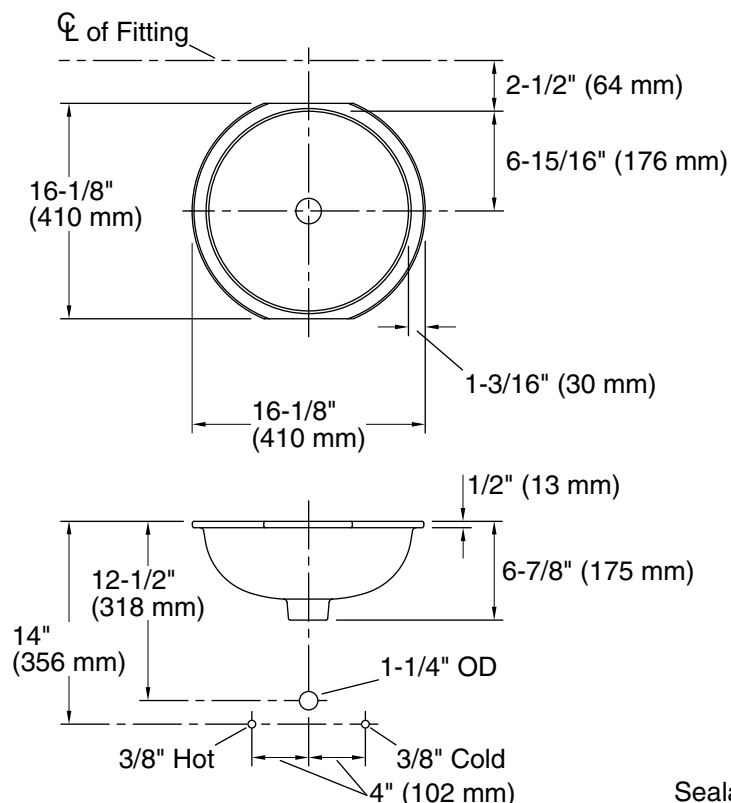
Standard Installation
