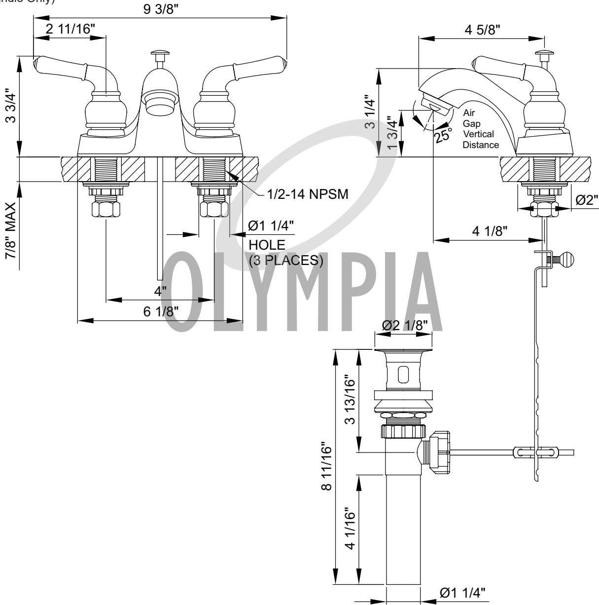
50/50 Pop-Up Drain
