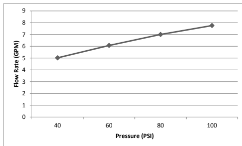
P-2306B Flow Rate (GPM) Vs Pressure (PSI) For Tub Port*
