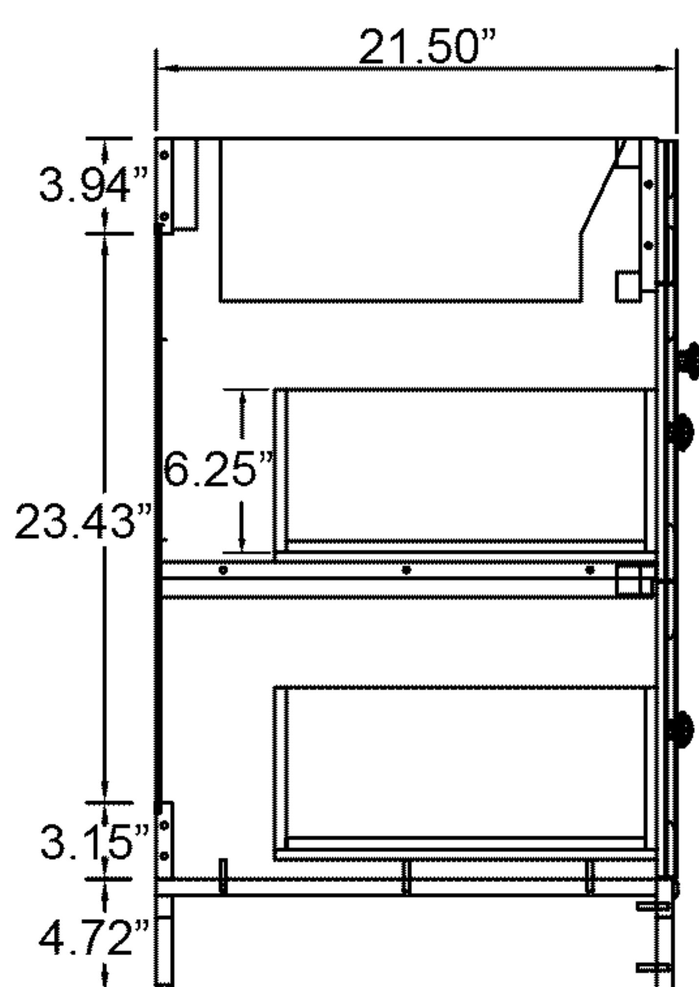
Side View
