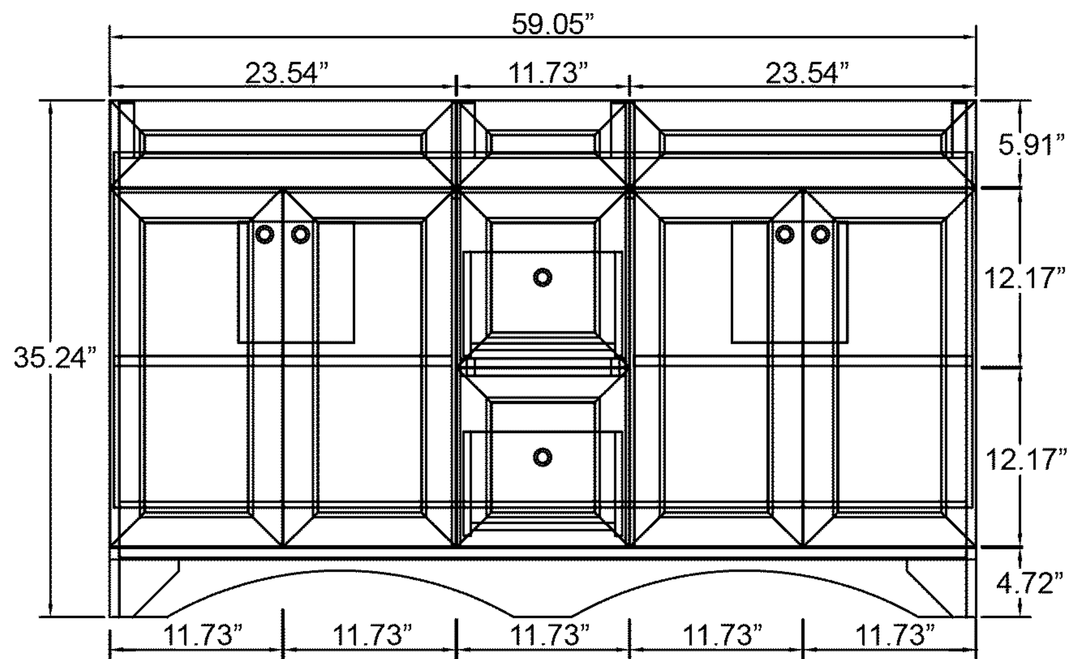
Front View
