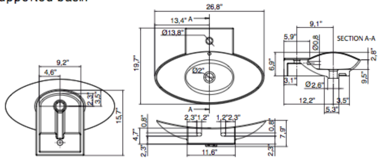
ZEFIRO 70/R 26,8" x 19,7" Art. 8204 Suspended or supported basin
