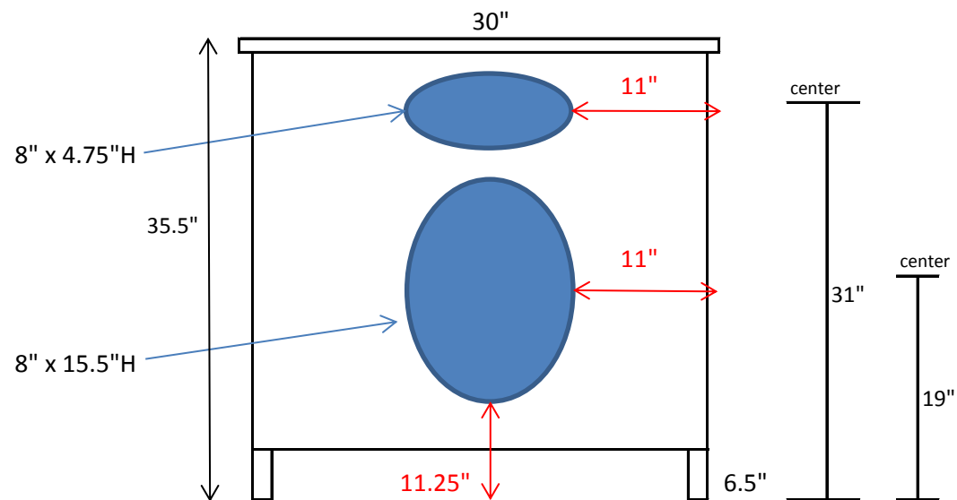
30" BWV-025 Ashley back cut out
