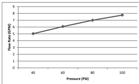
4023B Flow Rate (GPM) Vs Pressure (PSI)*
