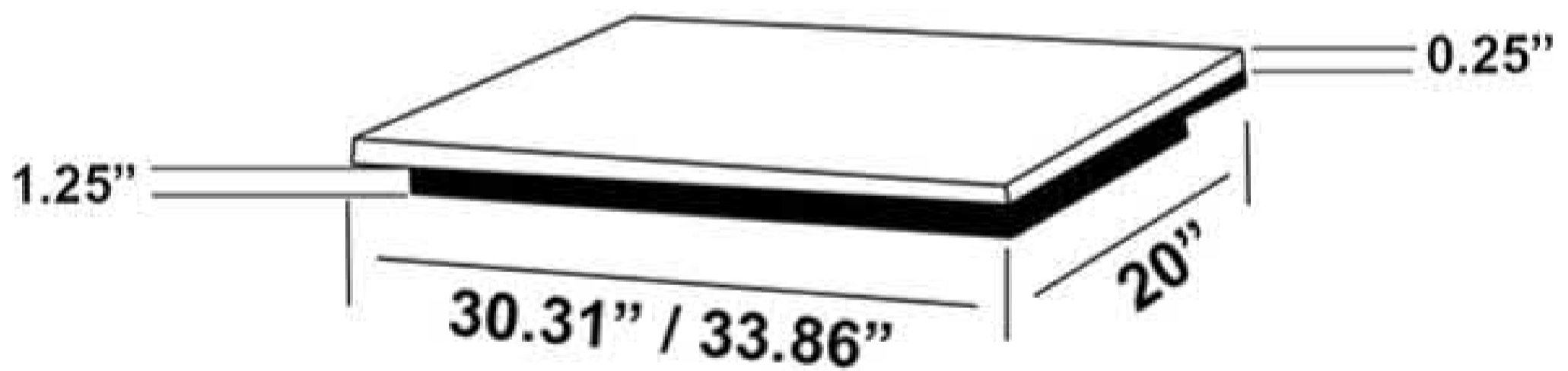
CUT-OUT VIEW
