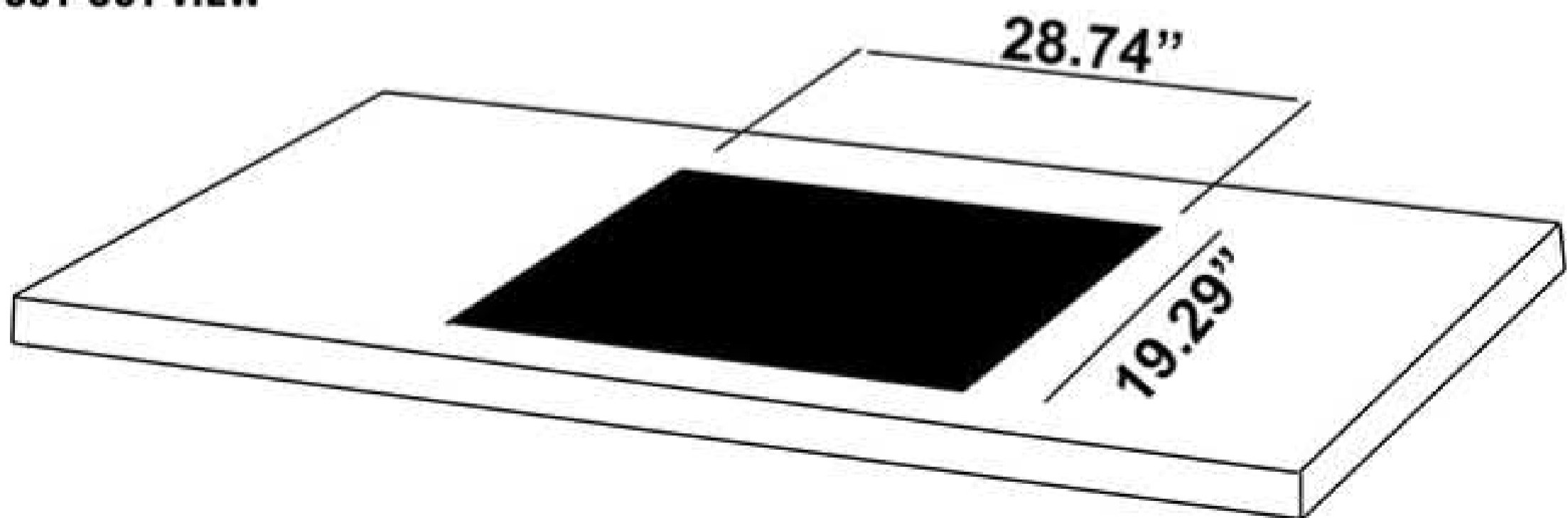
CUT-OUT VIEW
